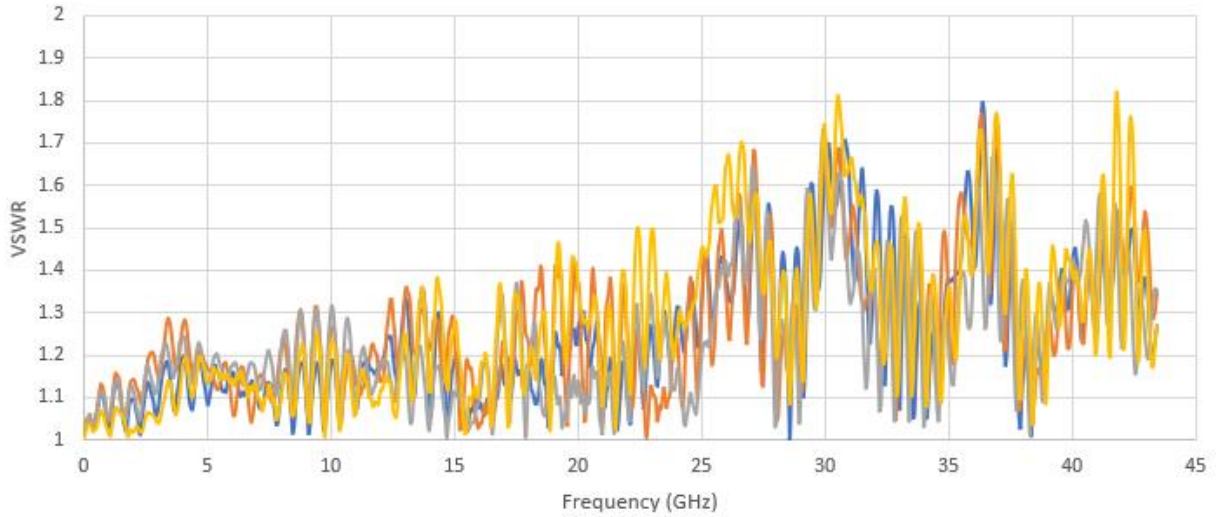
Typical VSWR vs Input Frequency (0 dBm reference level)
