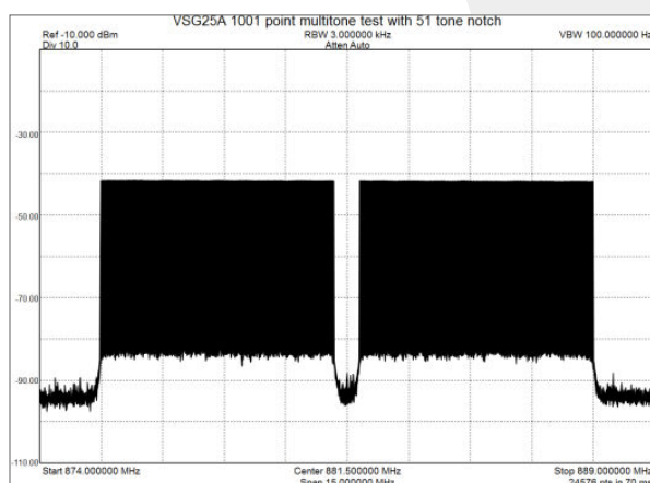
Figure 1—VSG25A test signal for NPR testing
